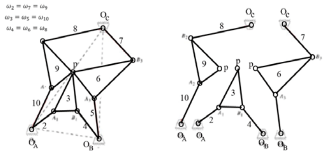
Fig. 7. Procedure of drawing cognates of a mechanism
