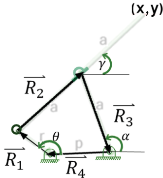
Fig. 3. Linkage notation
