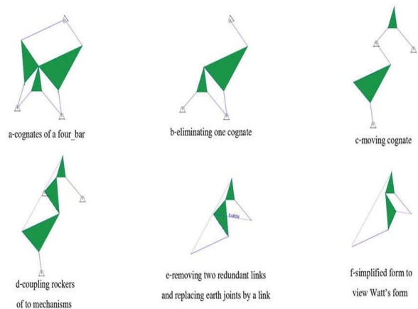
Fig. 9. Procedure of obtaining Watt six-bar linkage from optimal four-bar
