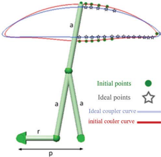
Fig. 5. Initial versus Ideal path
