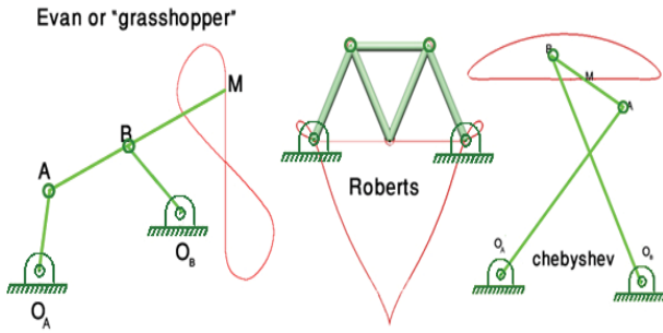
Fig. 1. Three known straight line generating mechanisms
