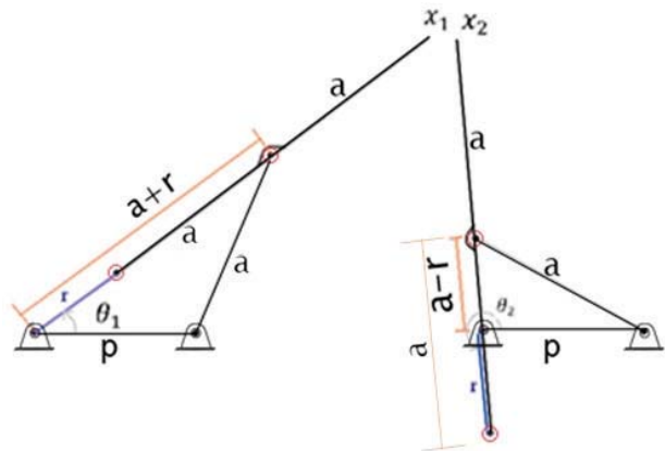
Fig. 4. Critical points and angles
