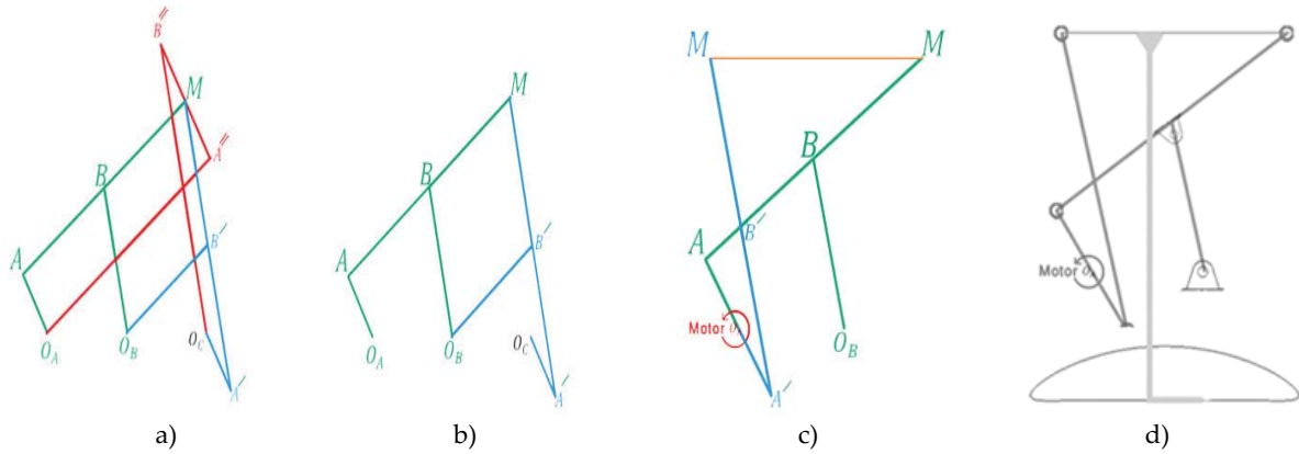
Fig. 10. Different stages of establishing the Watt's six-bar linkage with leg connected to straight and parallel moving link
