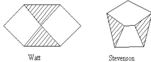
Fig. 8. Two basic kinematic chains belonging to the six-bar 1 degree of freedom class of mechanisms
